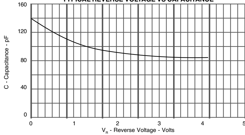
FIGURE 5 TYPICAL REVERSE VOLTAGE VS CAPACITANCE
